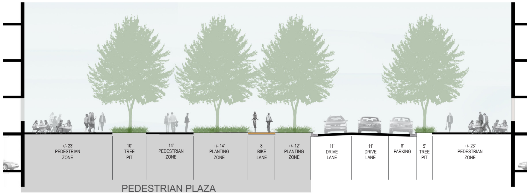
SECTION A
