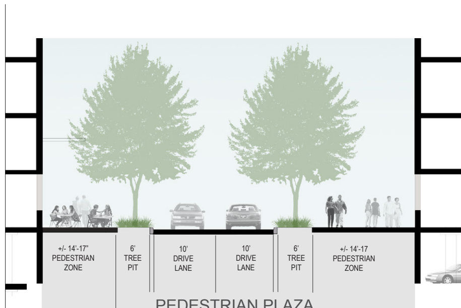
SECTION D
