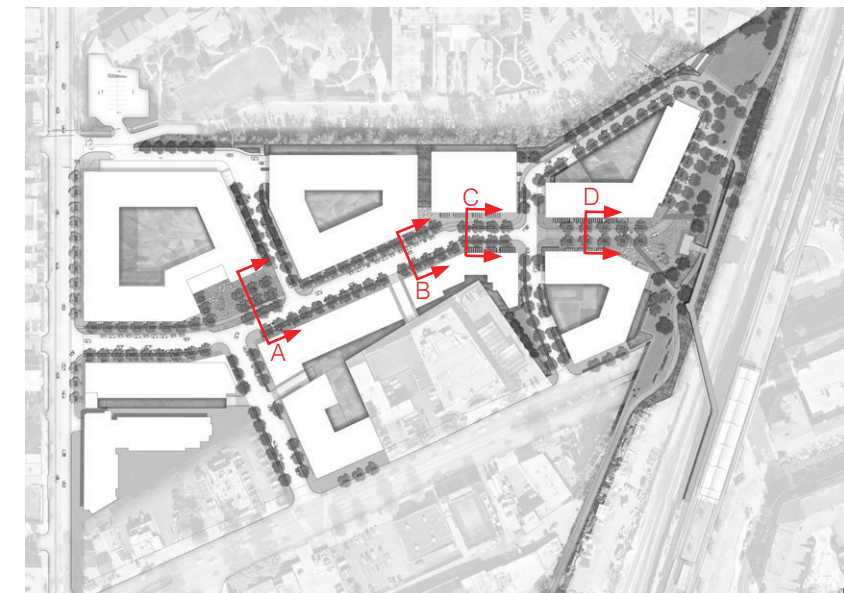
KEY PLAN
