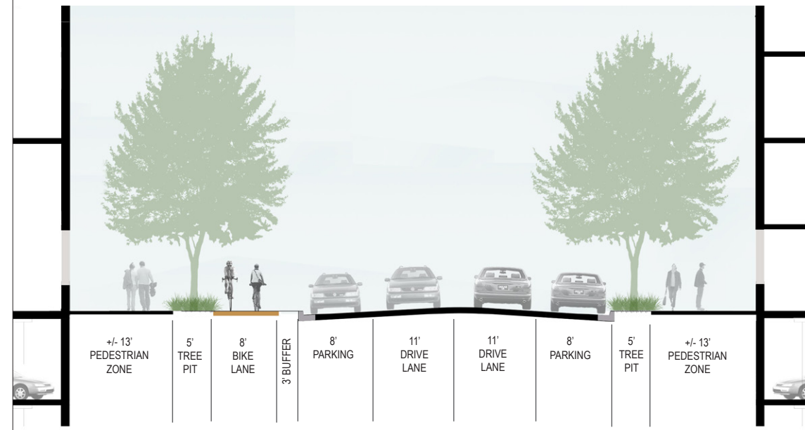
SECTION B
