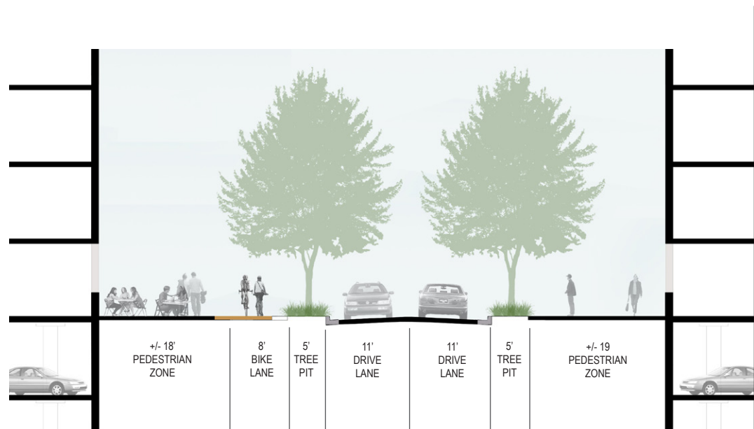
SECTION C
